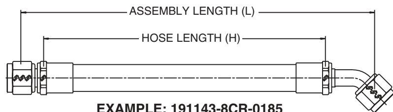
Straight-To-45° Elbow
